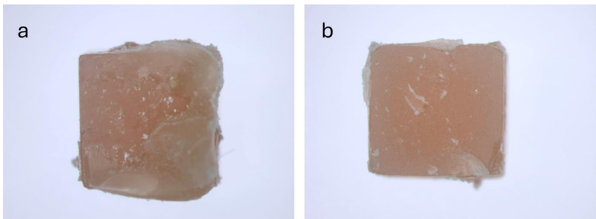
Figure: 3a Mixed Failure Between Liner And Denture Base Specimen. 3b Adhesive Failure Between Liner And Denture Base Specimen.
