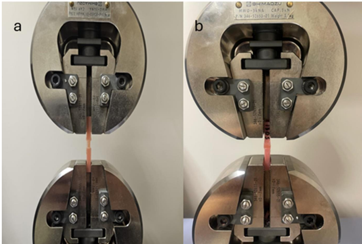
Figure: 2a Tensile Test on Soft Liner Applied Samples. 2b Tensile Test on Hard Liner Applied Samples.
