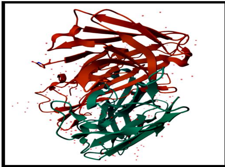
Figure 1. Crystal structure of Rituximab
