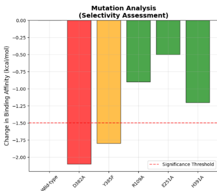
Figure 7. Mutation analysis
