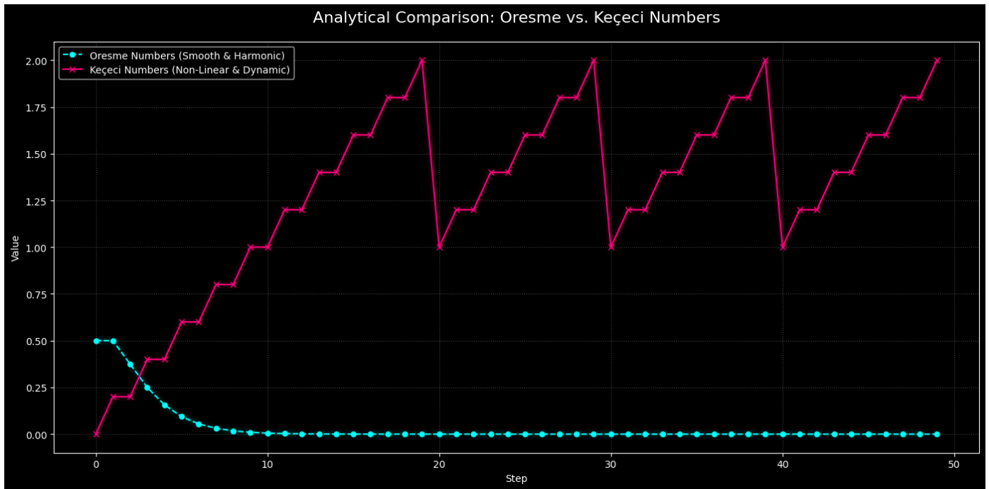
Figure 8: Analytical Comparison Oresme vs. Keçeci Numbers
